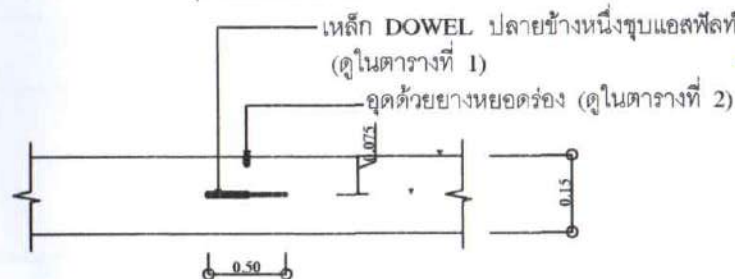
1 CONSTRUCTION JOINT
